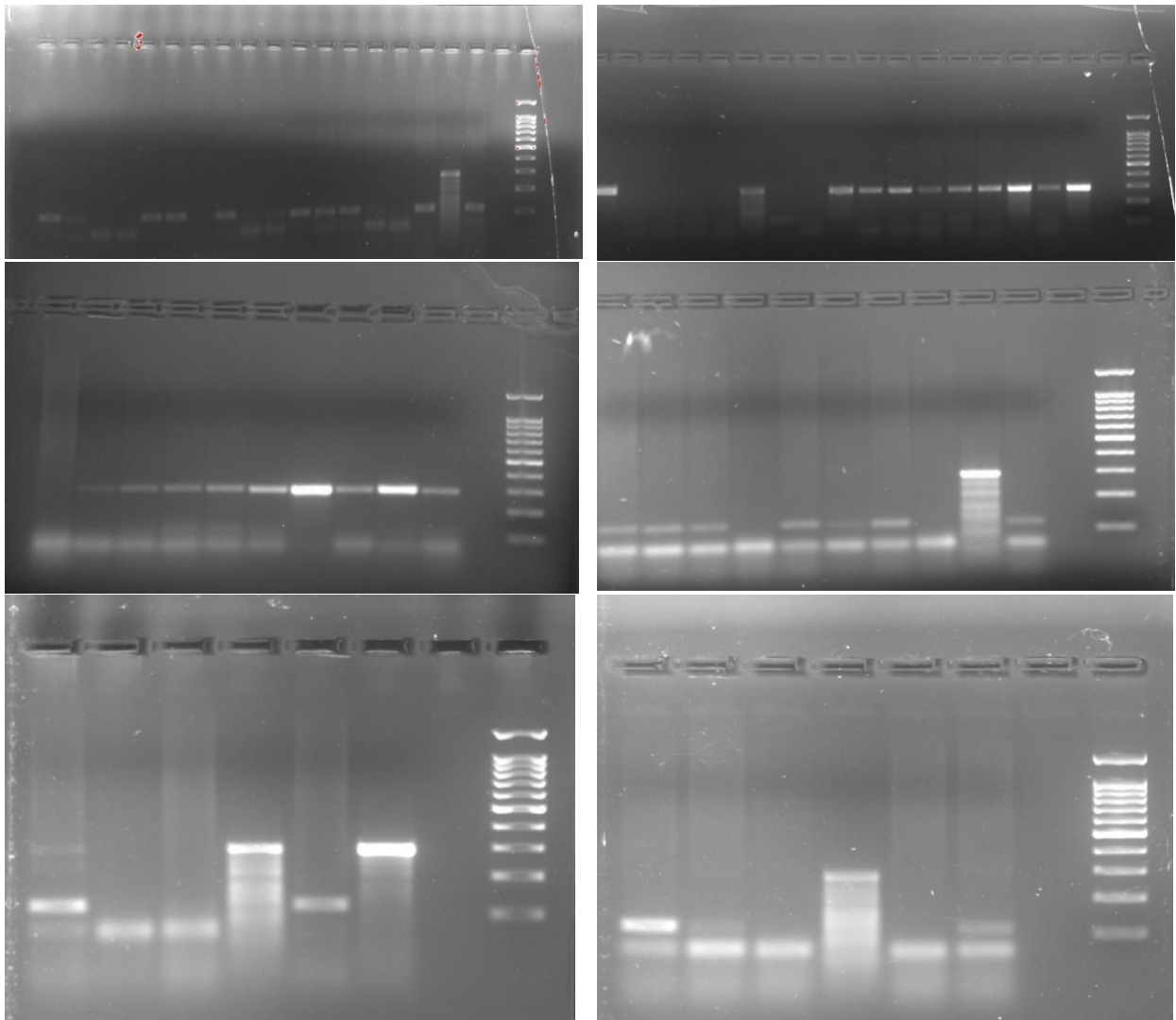
Figure S1. Amplicons of Salmonella spp. visualised on stained 1.5% agarose gels
