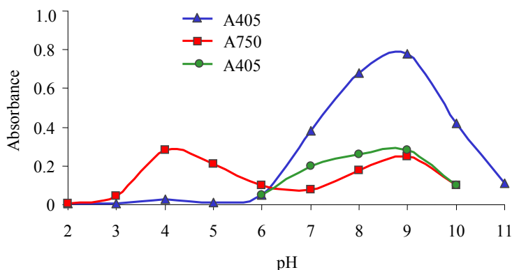
Figure 1. Effect of pH on the activity of larval proteinases and peptidases. The enzyme activity was determined to hemoglobin (red squares), L-BAPA (green circles) and L-Leu- p -NA (blue triangles) in buffers with different pH under conditions described in text. The following buffers of 100mM concentration were used: Glycine/HCl for pH 2–3, Citrate for pH 4–7, Tris/HCl for pH 8–9.5 and Glycine/NaOH for 10–11.5
