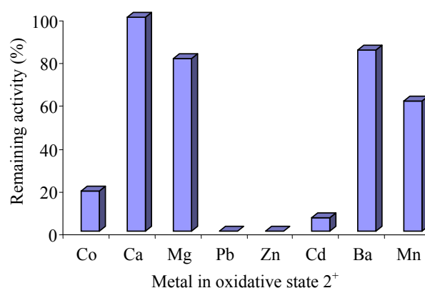
Figure 3. Effect of different metals on enzyme activity of supernatant fraction of first larval stadium. The metals were added to incubation solution in final concentration 1mM and enzyme activity was determined to L-Leu- p -NA under conditions described in text
