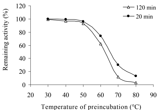
Figure 2. Effect of different temperatures on peptidolytic activity of supernatant fraction of first larval stadium. Enzymes were preincubated at 30°C, 40°C, 50°C, 60°C, 70°C and 80°C for 20 and 120 min and activity was determined to L-Leu- p -NA under conditions described in text
