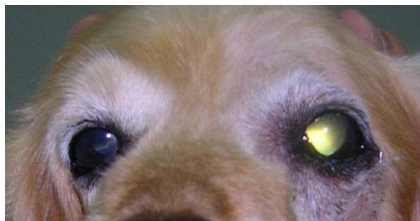
Figure 3. Tapetal reflection was seen but the retina was detached in the left eye in Case 8 (three weeks after operation)
