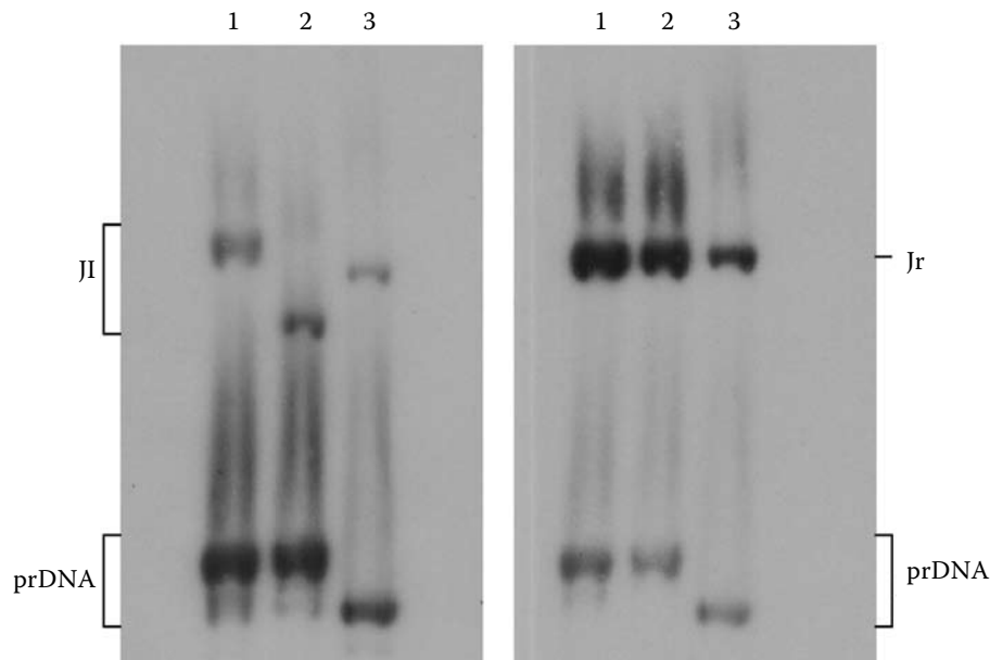
Figure 2. Southern blot hybridization of DNA of CH, Ni isolates and reference strain Movar 33/63 cleaved with Eco RI with the probes NiE22 and NiE50. The prDNA units, left junction (Jl) and right junction (Jr) fragments are indicated. Hybridization of A, the probe NiE22 (a) and probe NiE50 (b) with Eco RI digestion pattern of Movar 33/63, lane 1; isolate CH, lane 2 and Ni isolate, lane 3
